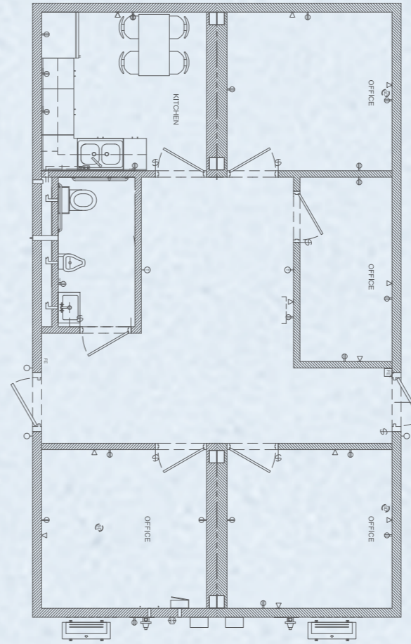
24 RKO 24W X 40L X 11H RESTROOM KITCHENETTE OFFICES
