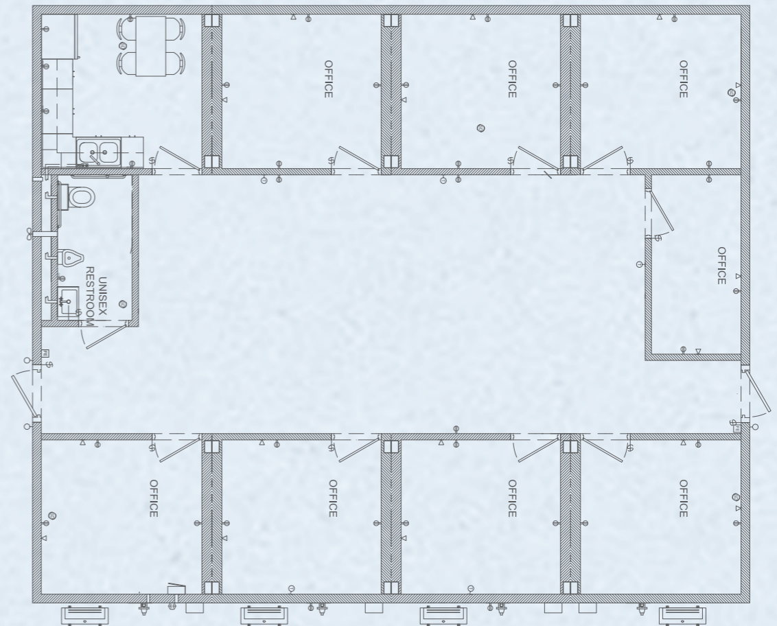
48 RKO 48W X 40L X 11H RESTROOM KITCHENETTE OFFICES
