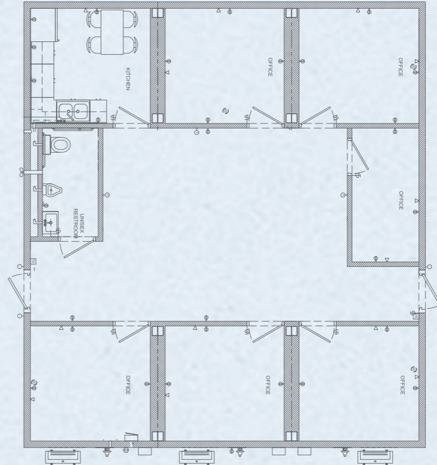
36 ··· RKO 36W X 40L X 11H RESTROOM KITCHENETTE OFFICES
